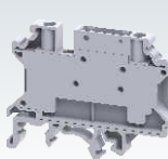
CF4SPFT 46 x 58.5 x 6 mm 0.2 - 4.0 mm 2 32 A, 1000 V, 0.5 Nm
