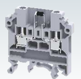
CKT4UD1/D2 46 x 46.3 x 6 mm 0.2 - 4.0 mm 2 1 A, 500 V, 0.5 Nm
