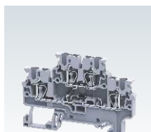
'CX' Series Ground / Earth Multiple Connection Terminal Blocks
