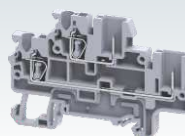
CXDL2.5/2B 48.7 x 78 x 5 mm 0.2 - 2.5 mm 2 24 A, 500 V
