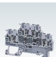
'CX' Series Ground / Earth Multiple Connection Terminal Blocks
