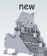
CYDLF4 90.1 x 94.5 x 6 mm 0.2 - 4.0 mm 2 10/32 A, 500 V, 0.5 Nm
