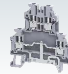
ODLG2.5 / ODLG2.5A 59.8 x 62 x 5 mm 0.2 - 2.5 mm 2 24 A, 800 V, 0.5 Nm
